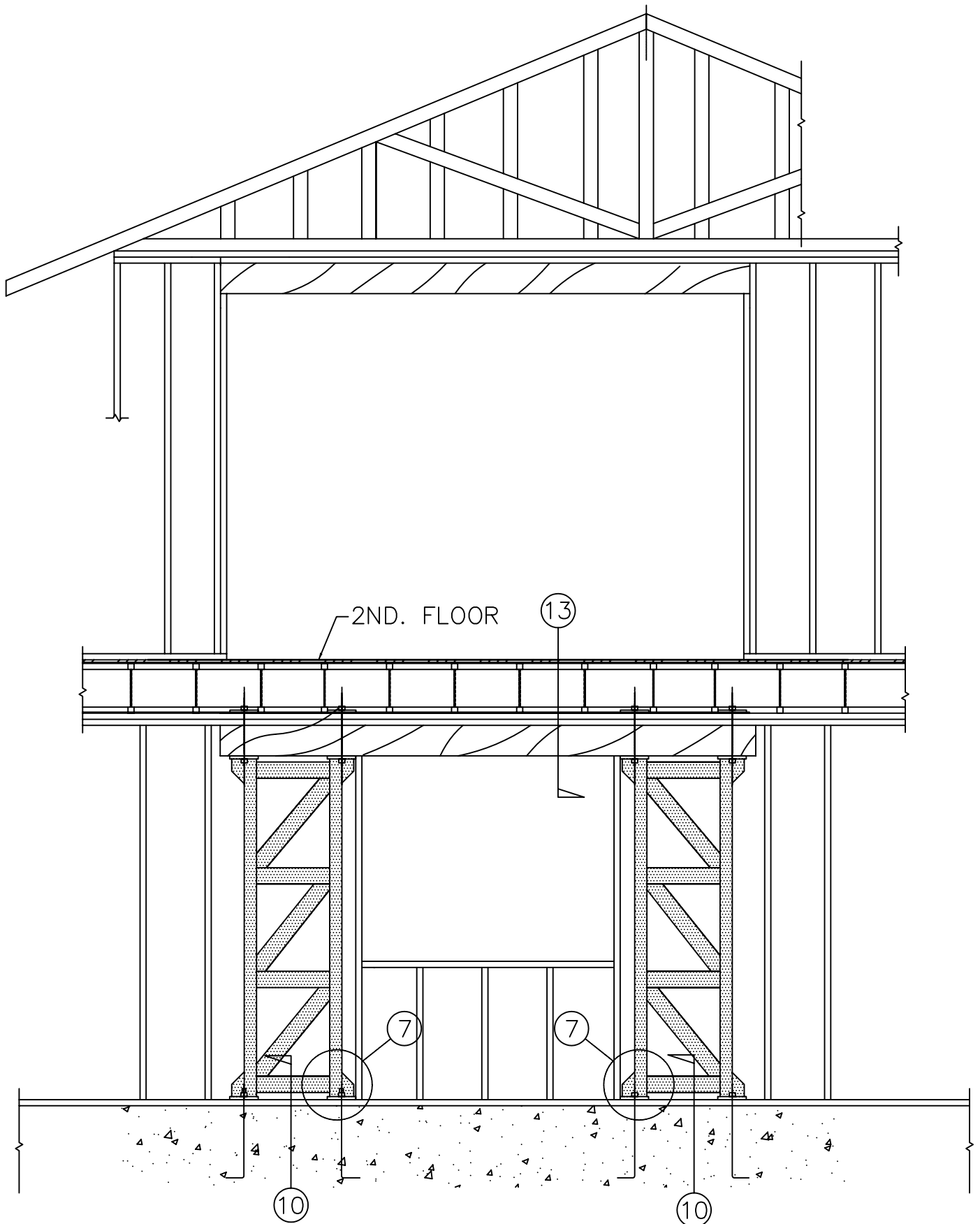
DROP BEAM @ 2ND. FLOOR SCALE: N.T.S.
