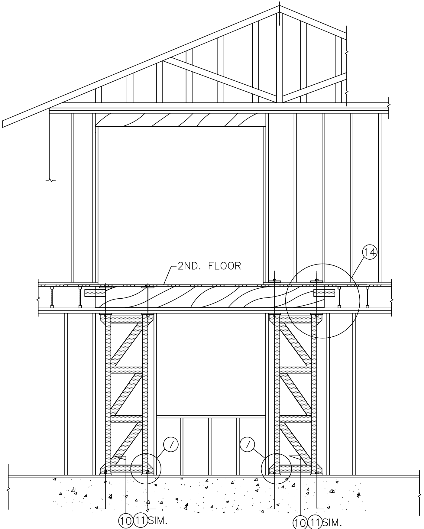
FLUSH BEAM @ 2ND. FLOOR SCALE: N.T.S.
