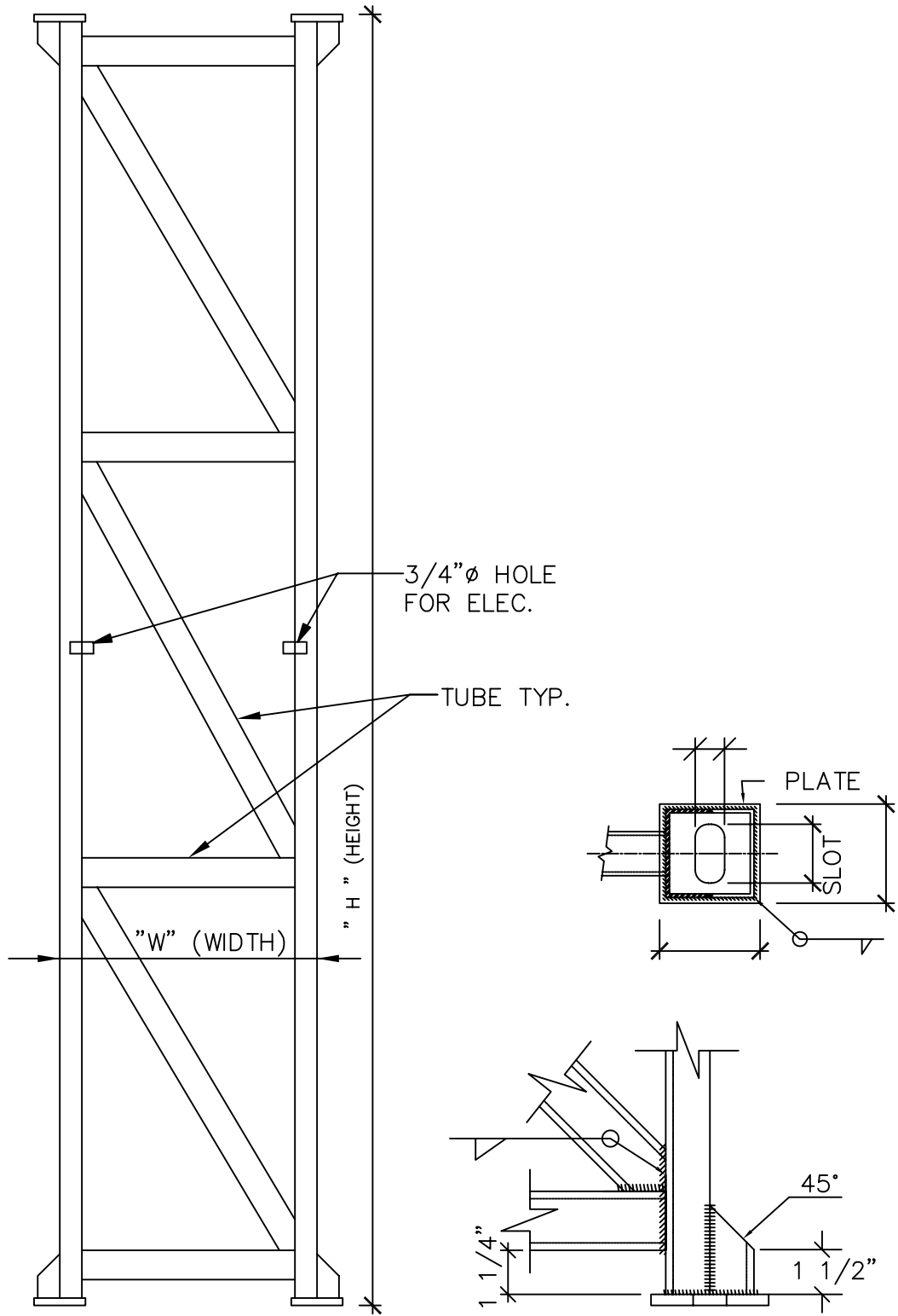
9 TYP. BRACED FRAME ELEVATION
